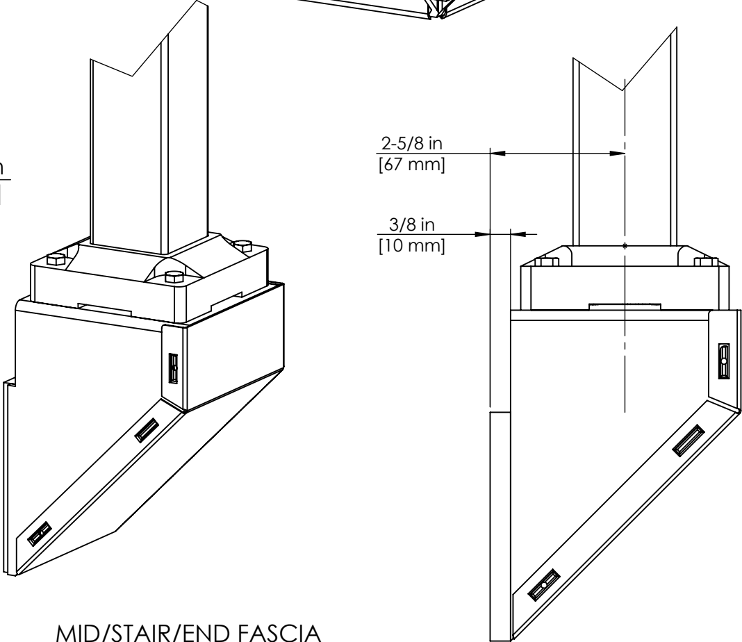
MID/STAIR/END FASCIA MOUNT BRACKET
